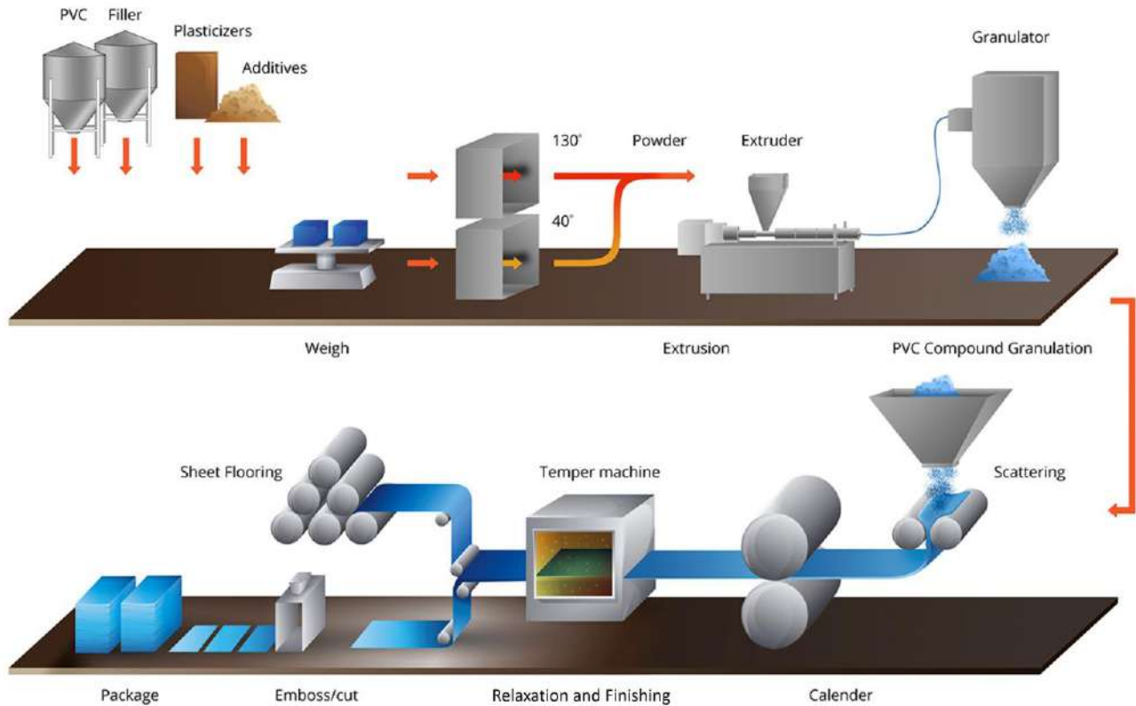
Example of Production Line for Homogeneous Sheet Vinyl Flooring
