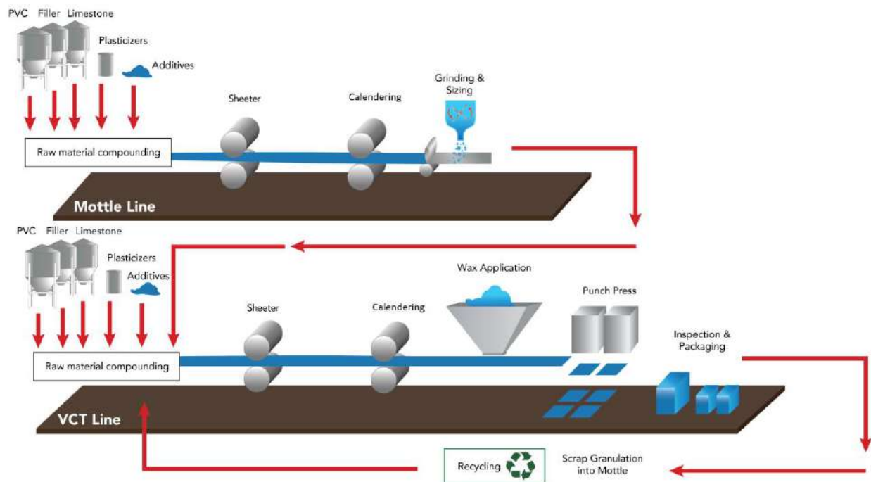
Example of Production Line for VCT Flooring
